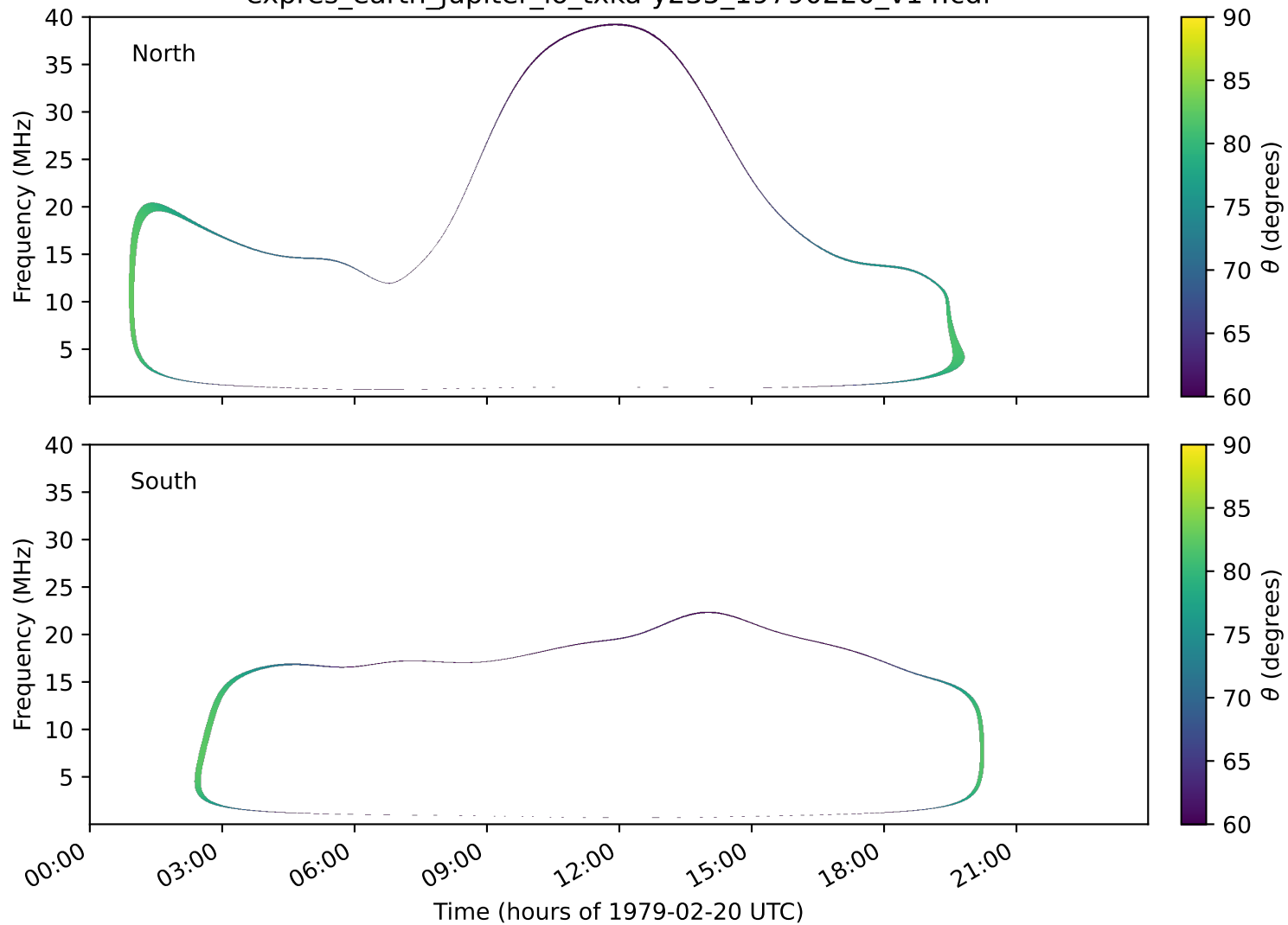
expres_earth_jupiter_io_txka-y235_19790220_v14.cdf
