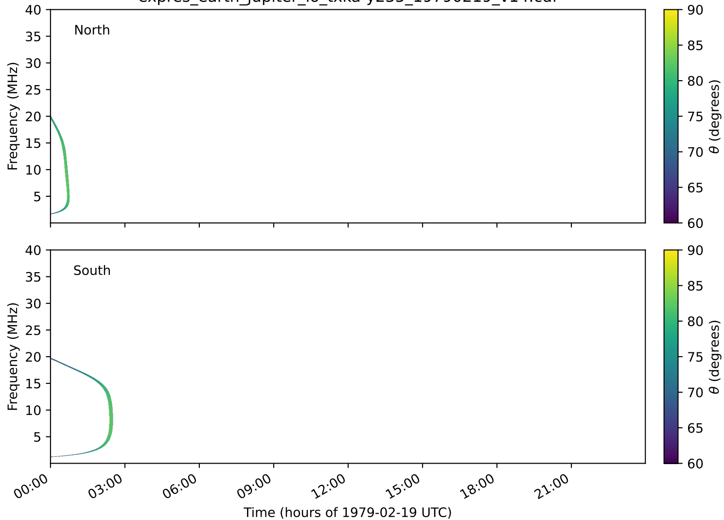
expres_earth_jupiter_io_txka-y235_19790219_v14.cdf
