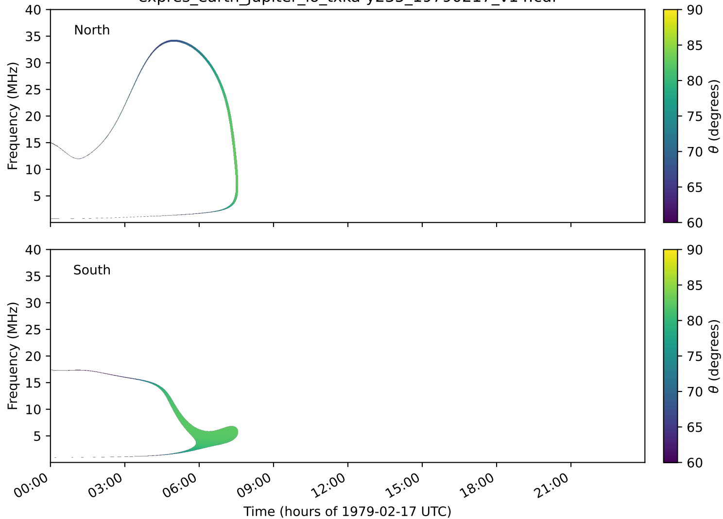
expres_earth_jupiter_io_txka-y235_19790217_v14.cdf
