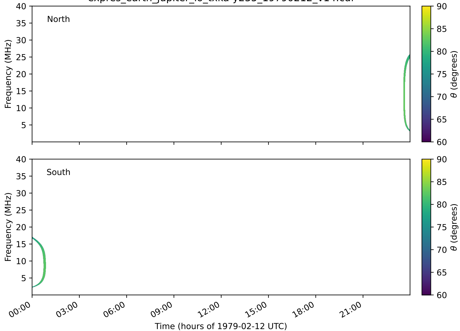
expres_earth_jupiter_io_txka-y235_19790212_v14.cdf
