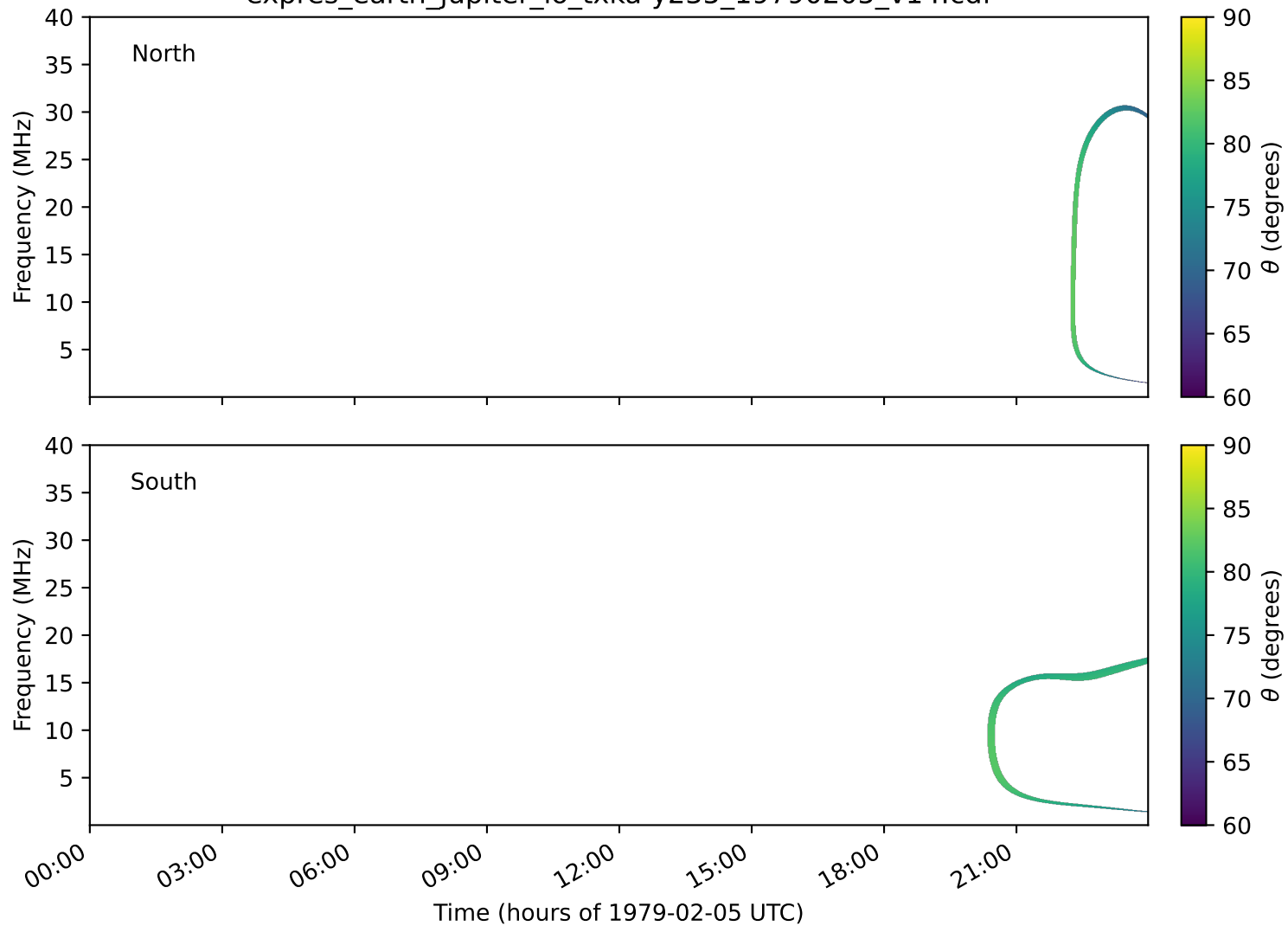
expres_earth_jupiter_io_txka-y235_19790205_v14.cdf
