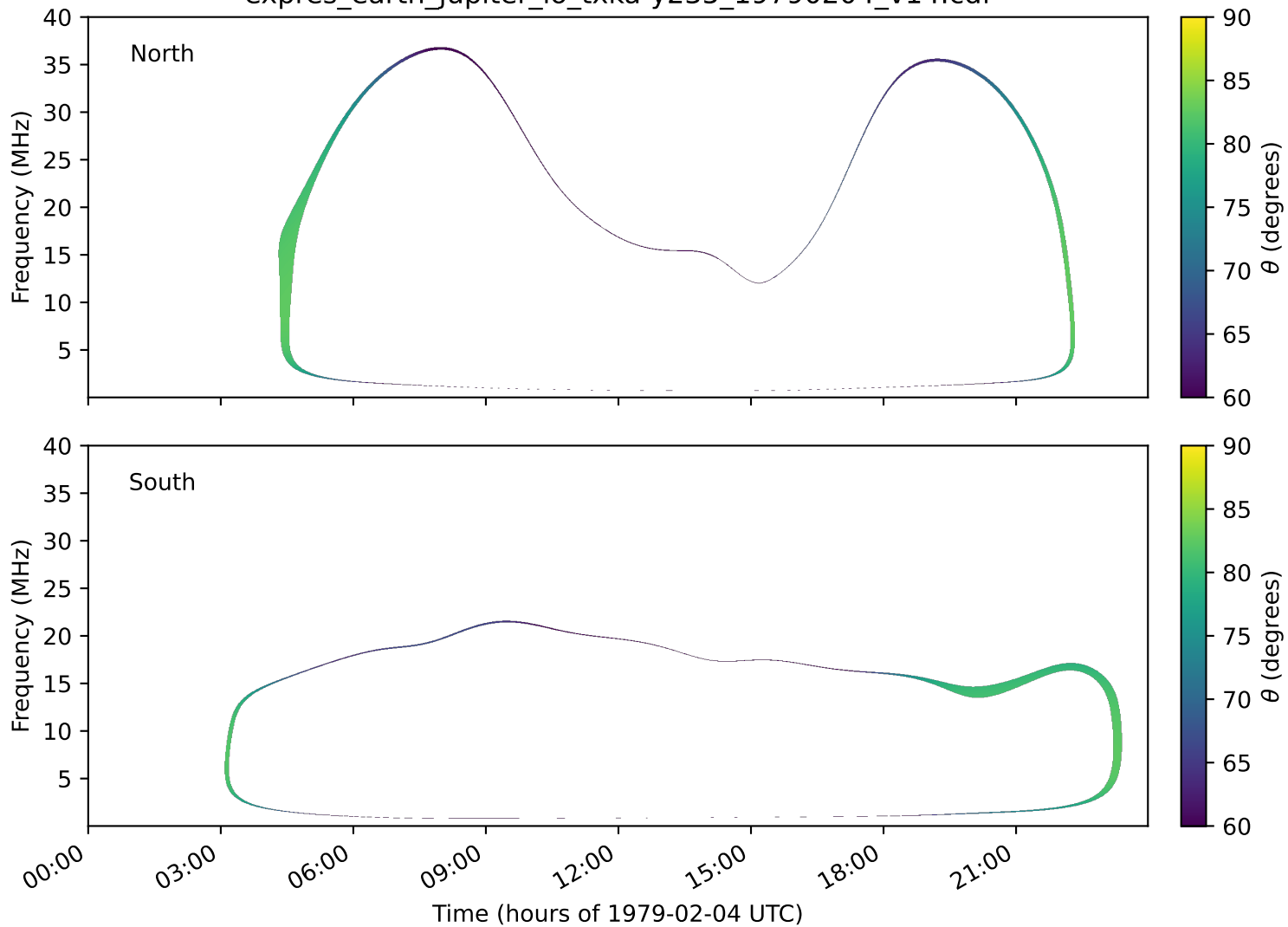
expres_earth_jupiter_io_txka-y235_19790204_v14.cdf
