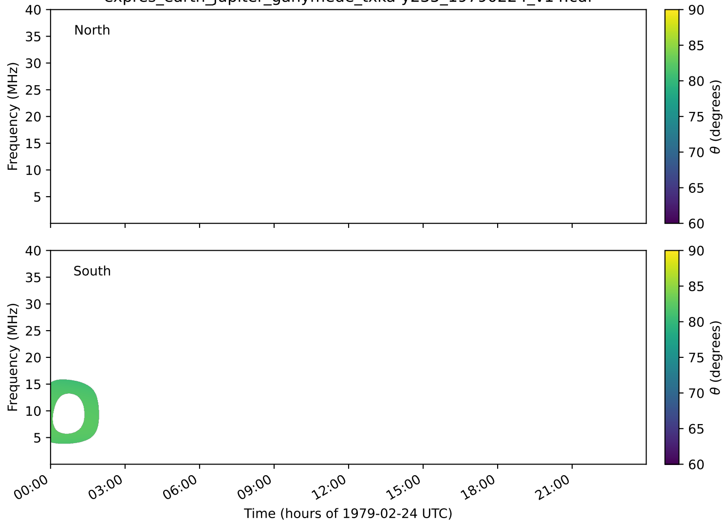
expres_earth_jupiter_ganymede_txka-y235_19790224_v14.cdf
