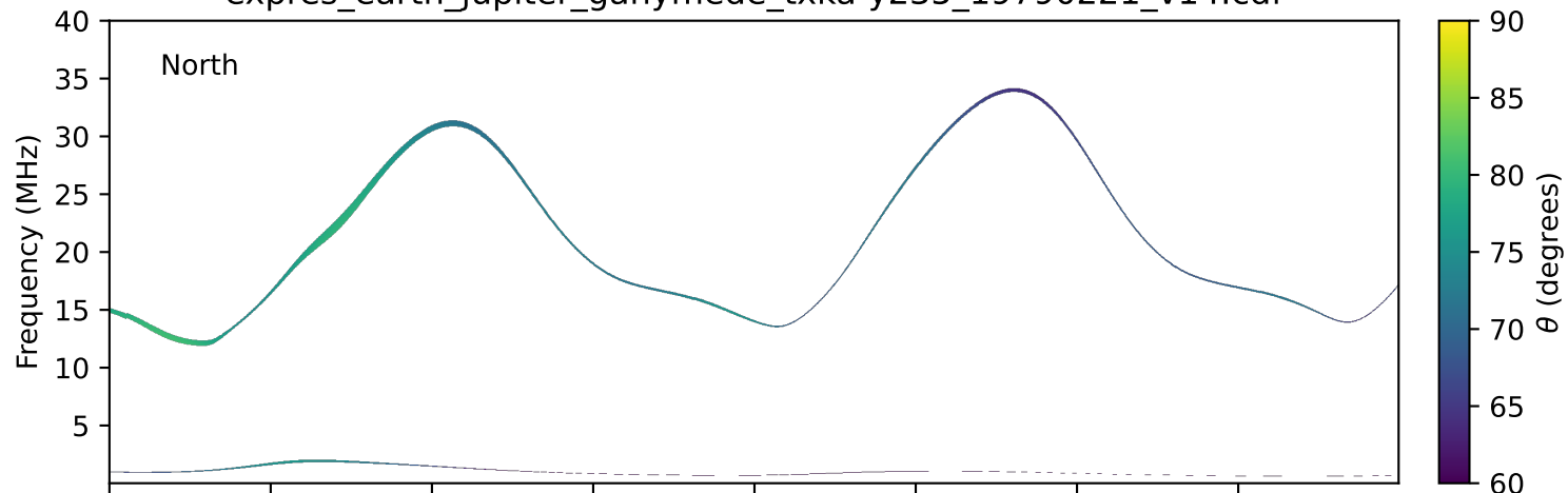
expres_earth_jupiter_ganymede_txka-y235_19790221_v14.cdf
