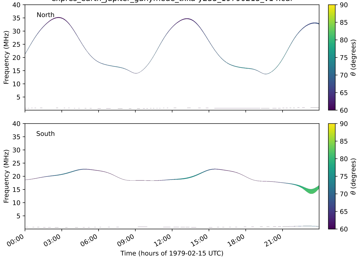
expres_earth_jupiter_ganymede_txka-y235_19790215_v14.cdf
