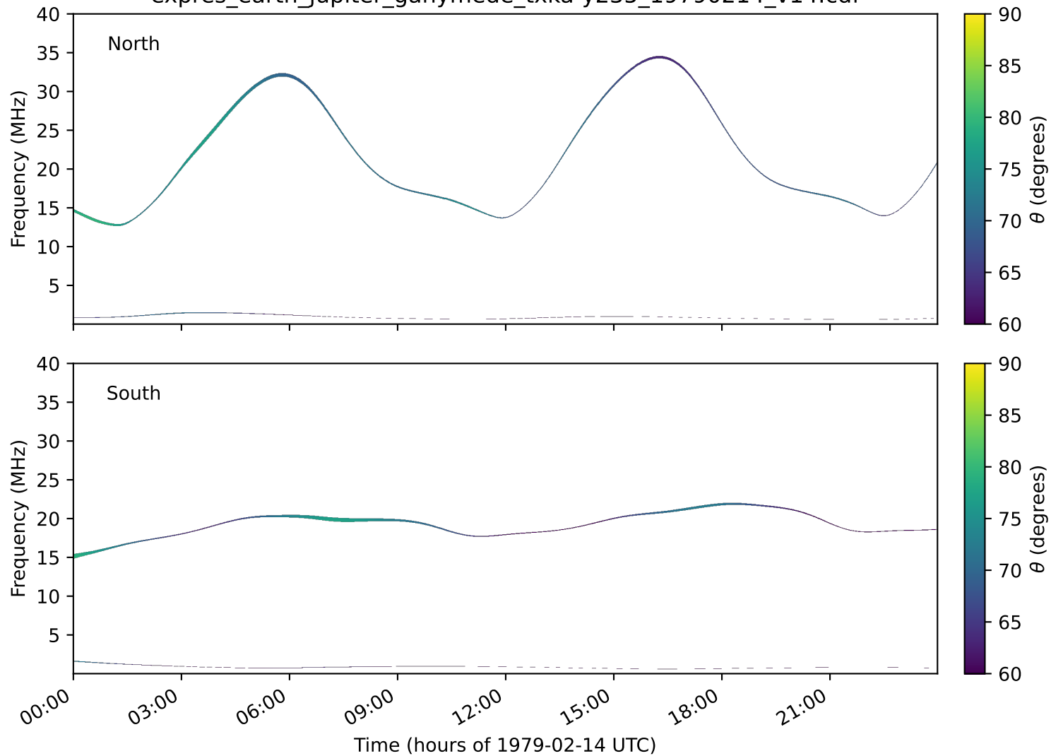
expres_earth_jupiter_ganymede_txka-y235_19790214_v14.cdf
