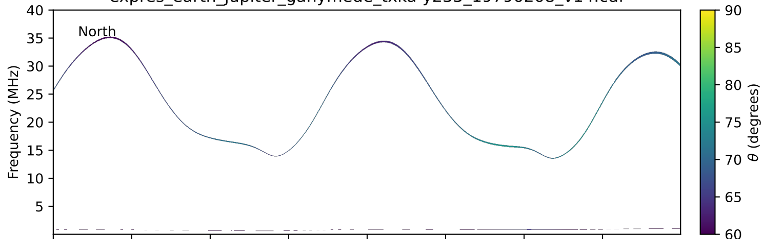
expres_earth_jupiter_ganymede_txka-y235_19790208_v14.cdf
