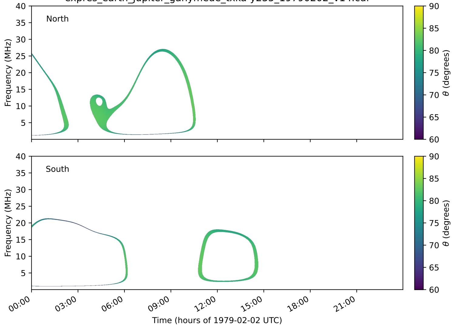
expres_earth_jupiter_ganymede_txka-y235_19790202_v14.cdf
