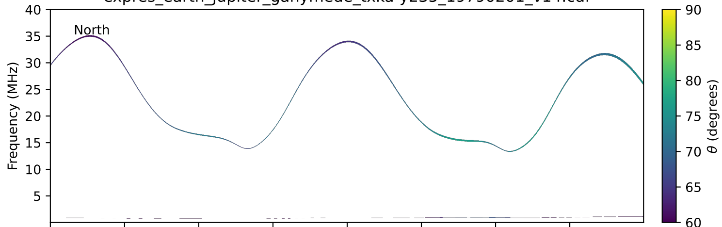
expres_earth_jupiter_ganymede_txka-y235_19790201_v14.cdf
