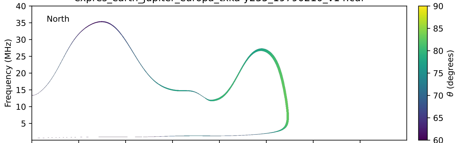
expres_earth_jupiter_europa_txka-y235_19790210_v14.cdf
