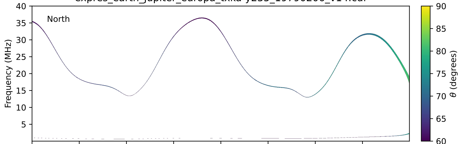
expres_earth_jupiter_europa_txka-y235_19790206_v14.cdf
