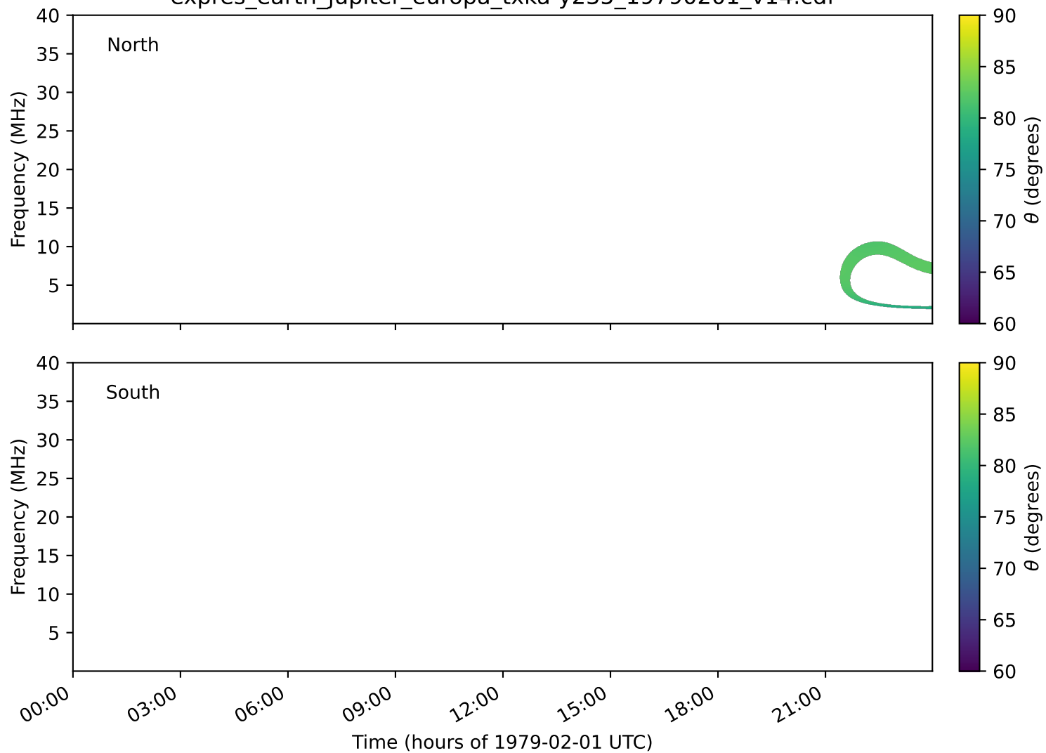
expres_earth_jupiter_europa_txka-y235_19790201_v14.cdf
