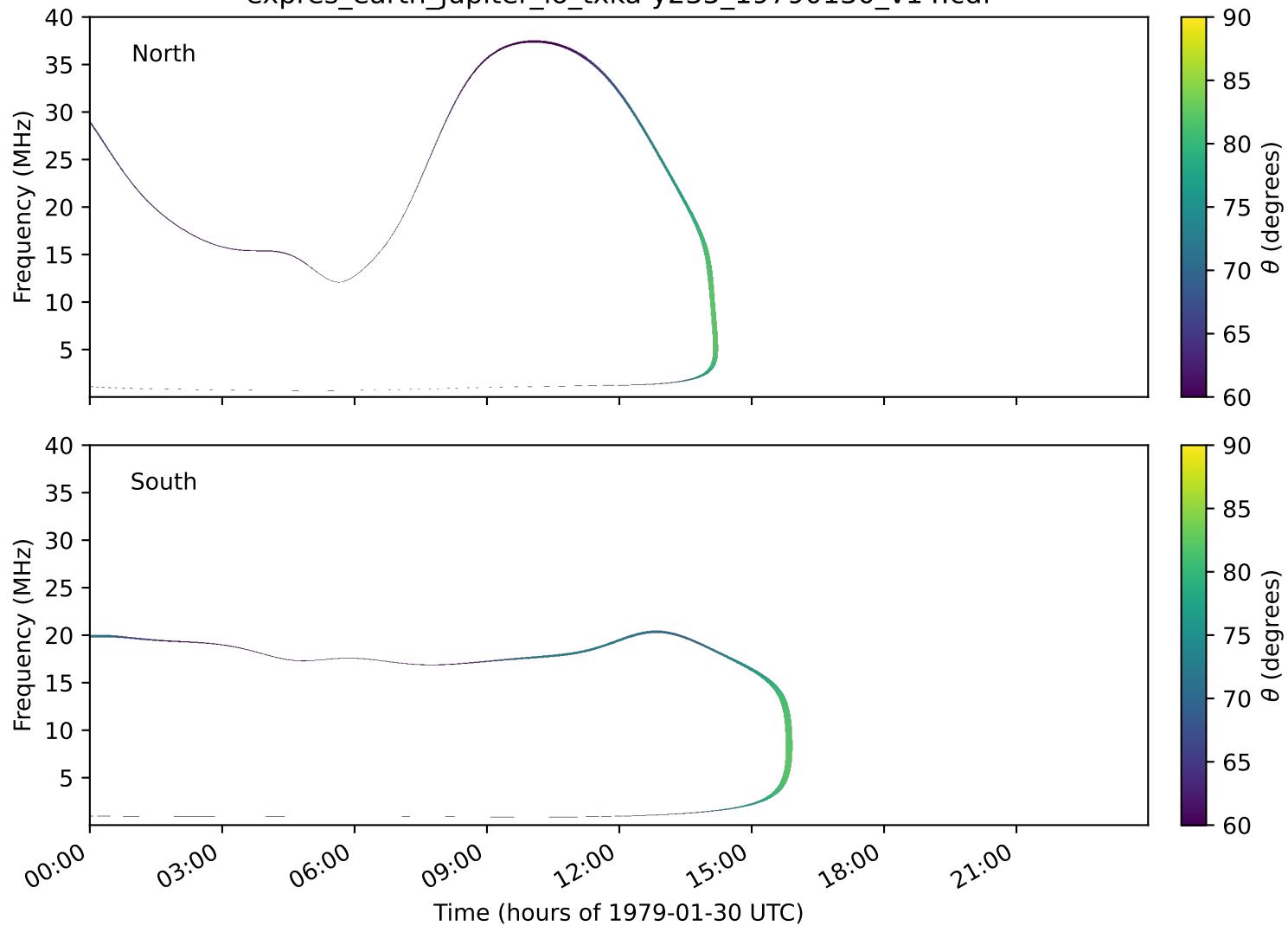
expres_earth_jupiter_io_txka-y235_19790130_v14.cdf
