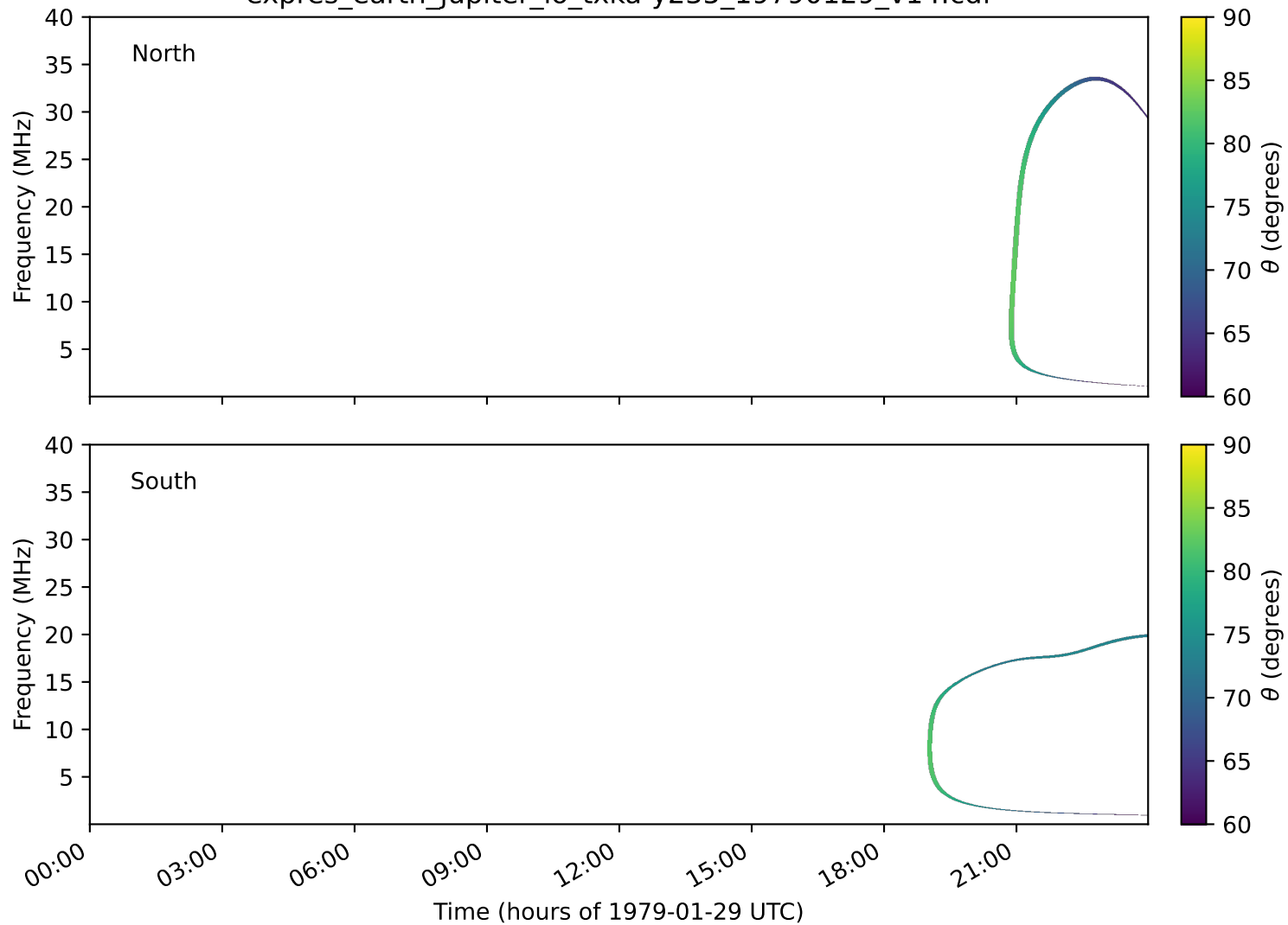
expres_earth_jupiter_io_txka-y235_19790129_v14.cdf
