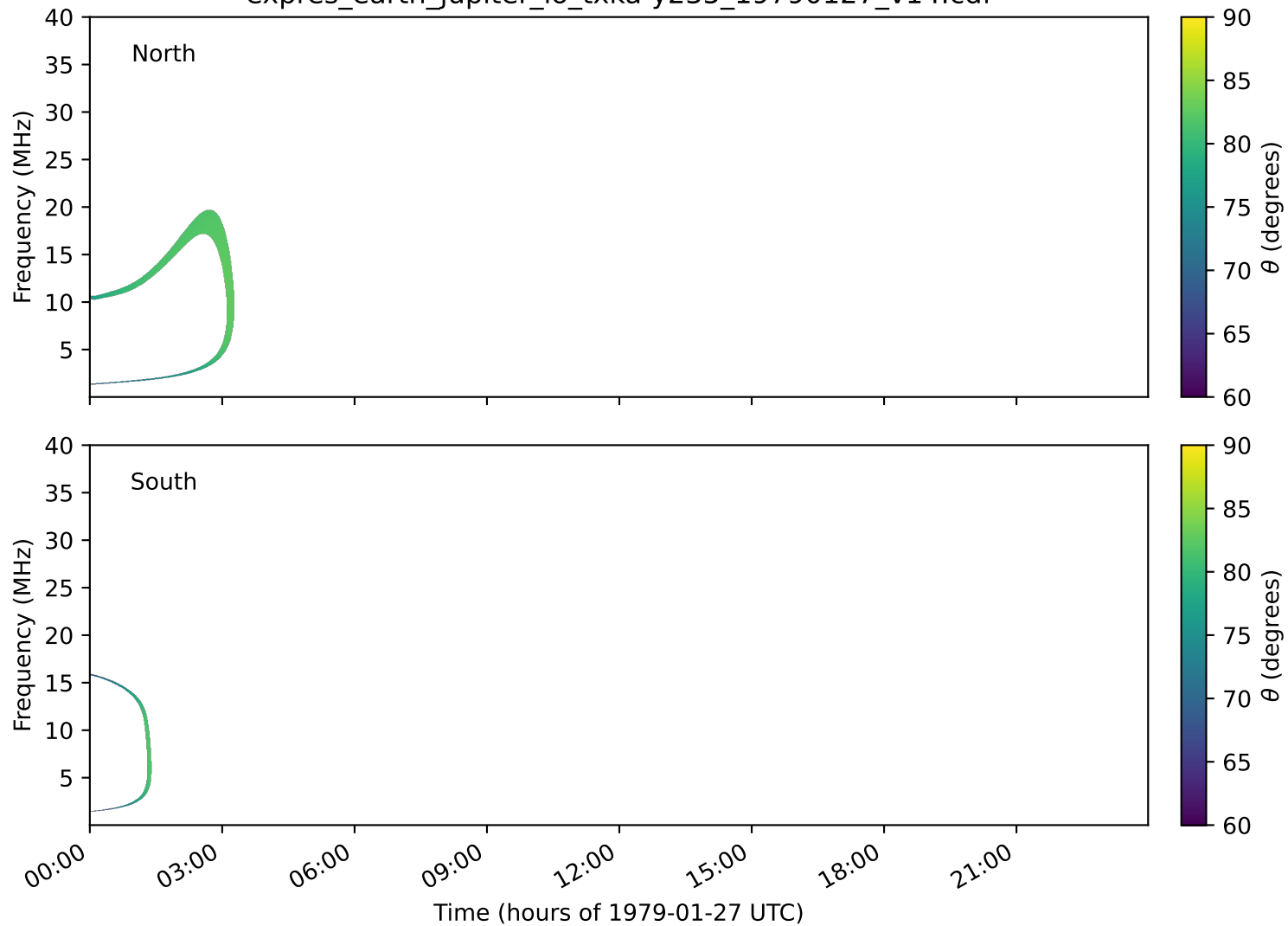
expres_earth_jupiter_io_txka-y235_19790127_v14.cdf
