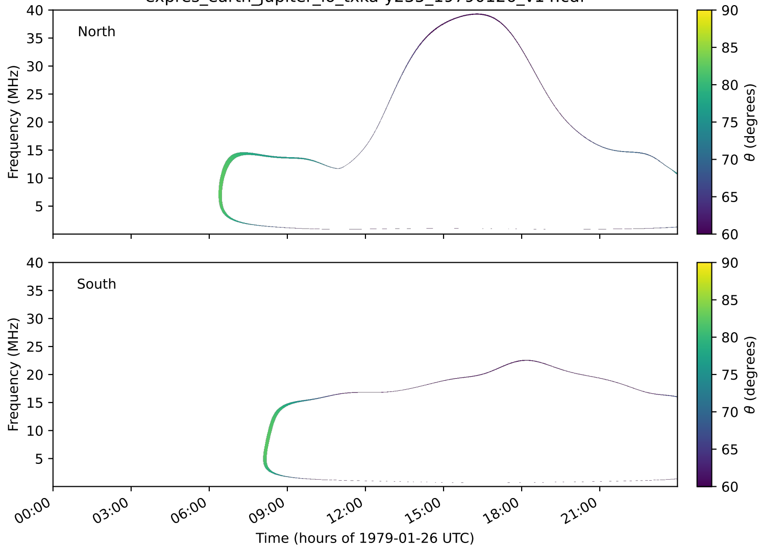
expres_earth_jupiter_io_txka-y235_19790126_v14.cdf
