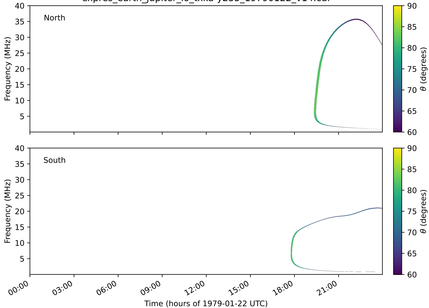
expres_earth_jupiter_io_txka-y235_19790122_v14.cdf
