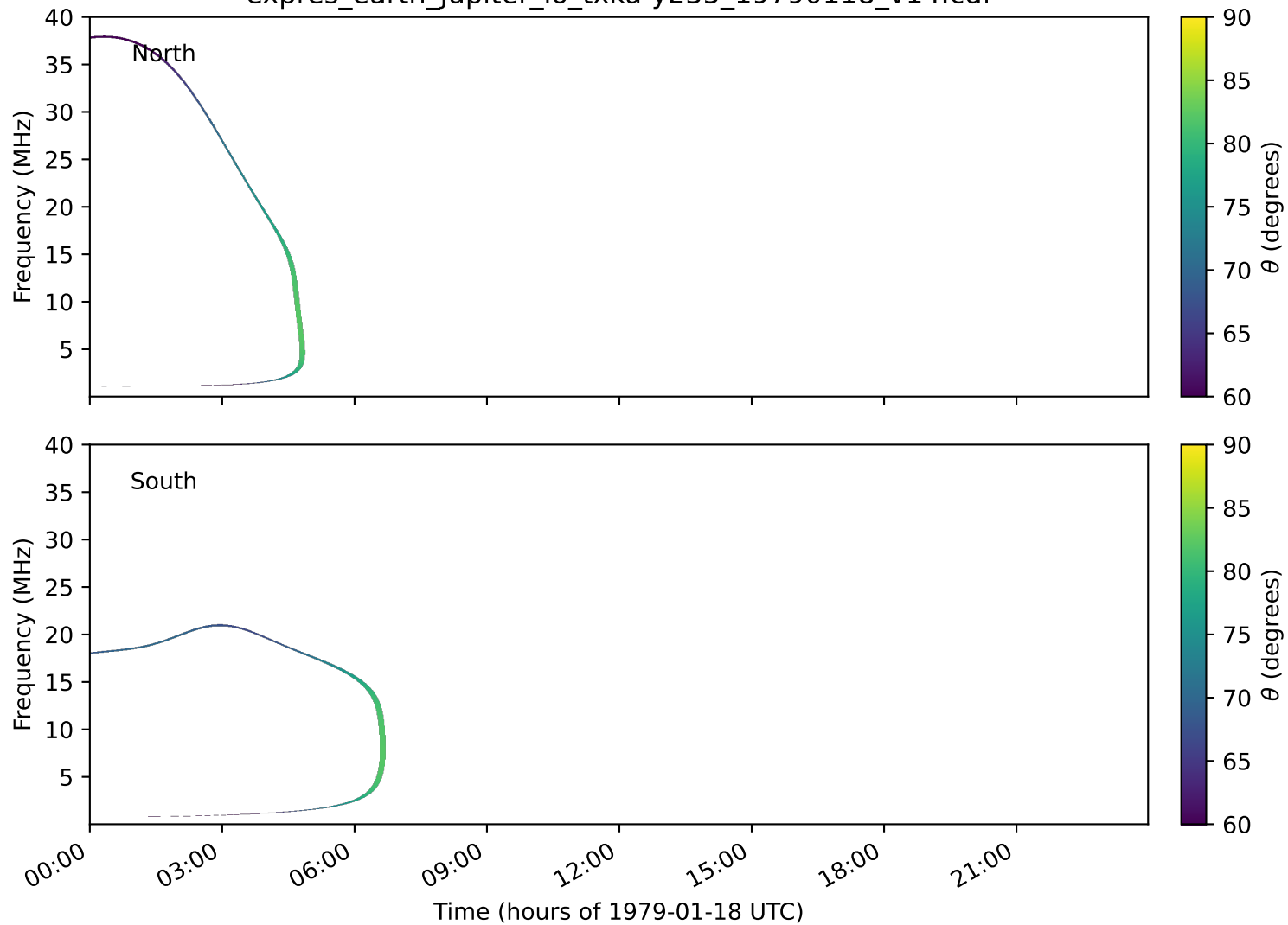
expres_earth_jupiter_io_txka-y235_19790118_v14.cdf
