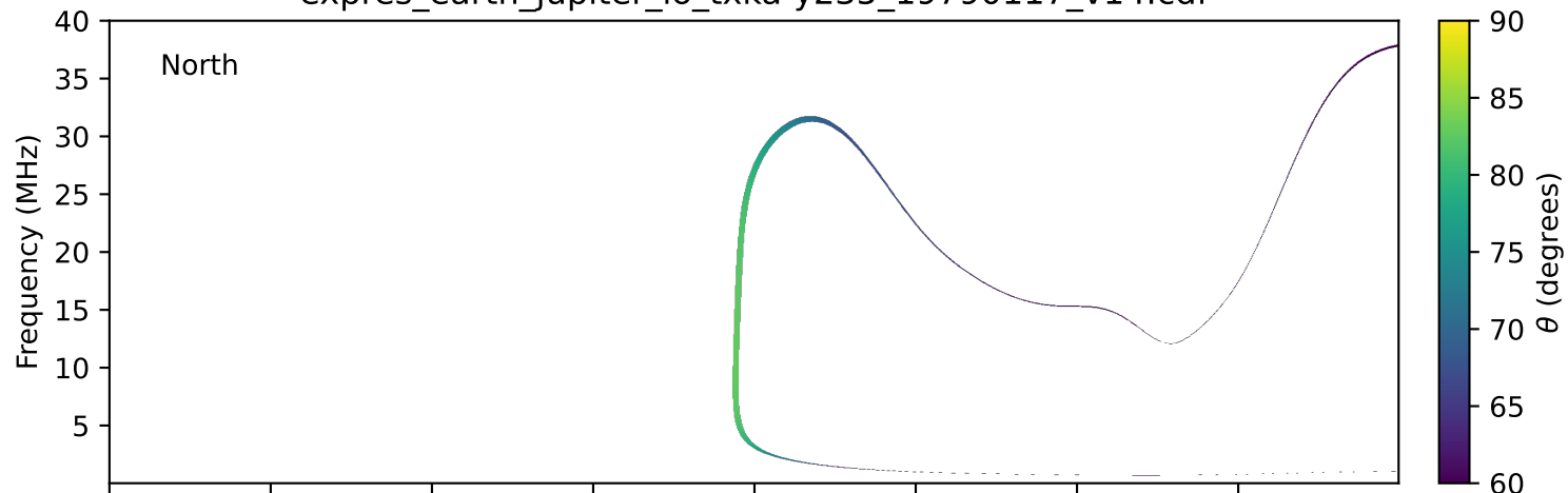
expres_earth_jupiter_io_txka-y235_19790117_v14.cdf
