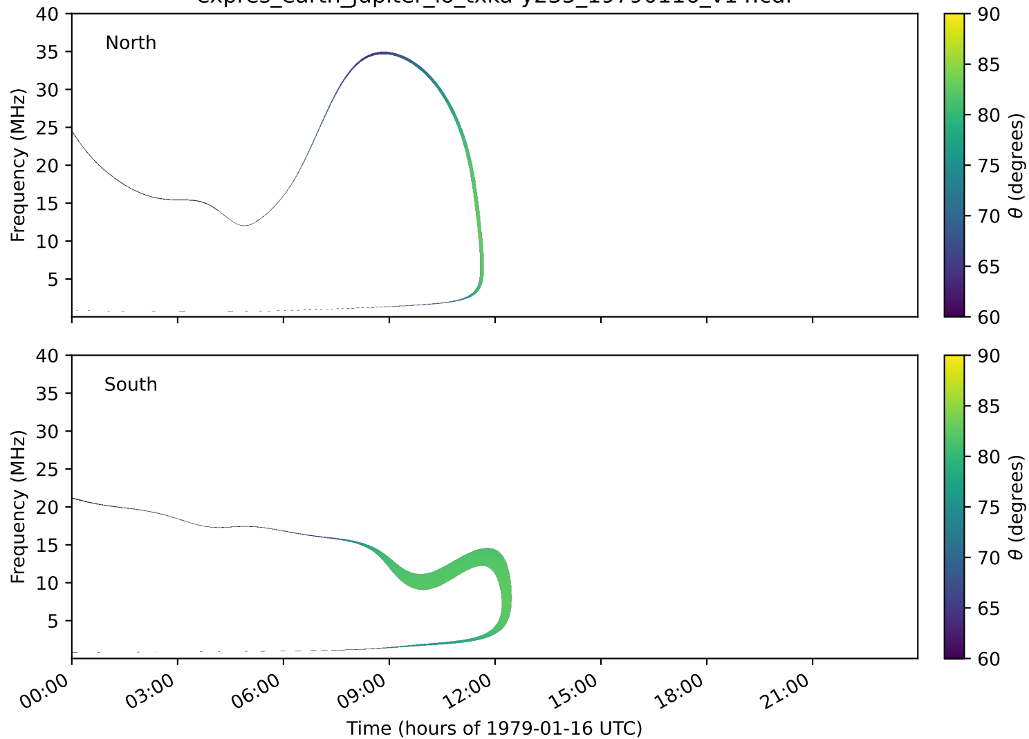
expres_earth_jupiter_io_txka-y235_19790116_v14.cdf
