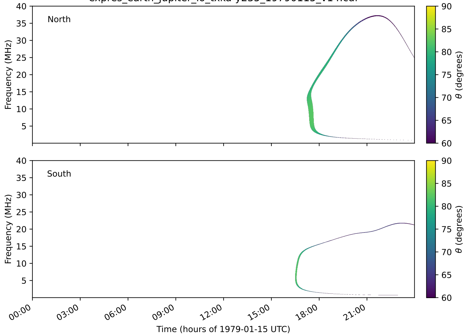
expres_earth_jupiter_io_txka-y235_19790115_v14.cdf
