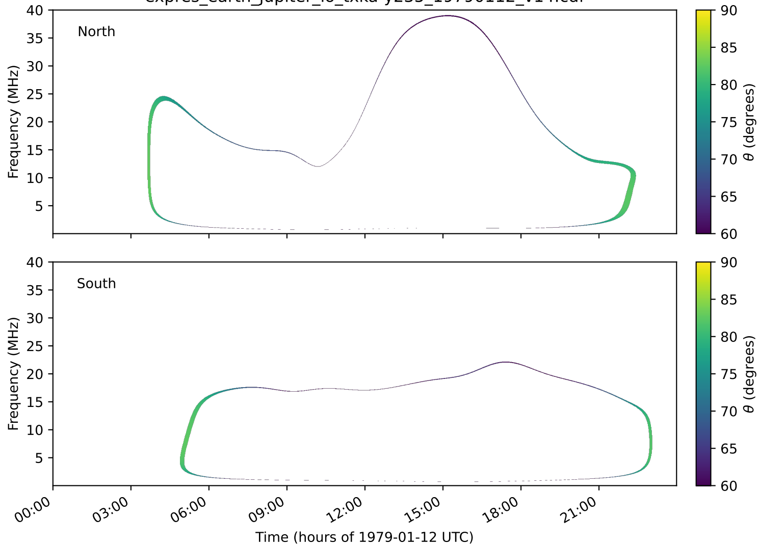
expres_earth_jupiter_io_txka-y235_19790112_v14.cdf
