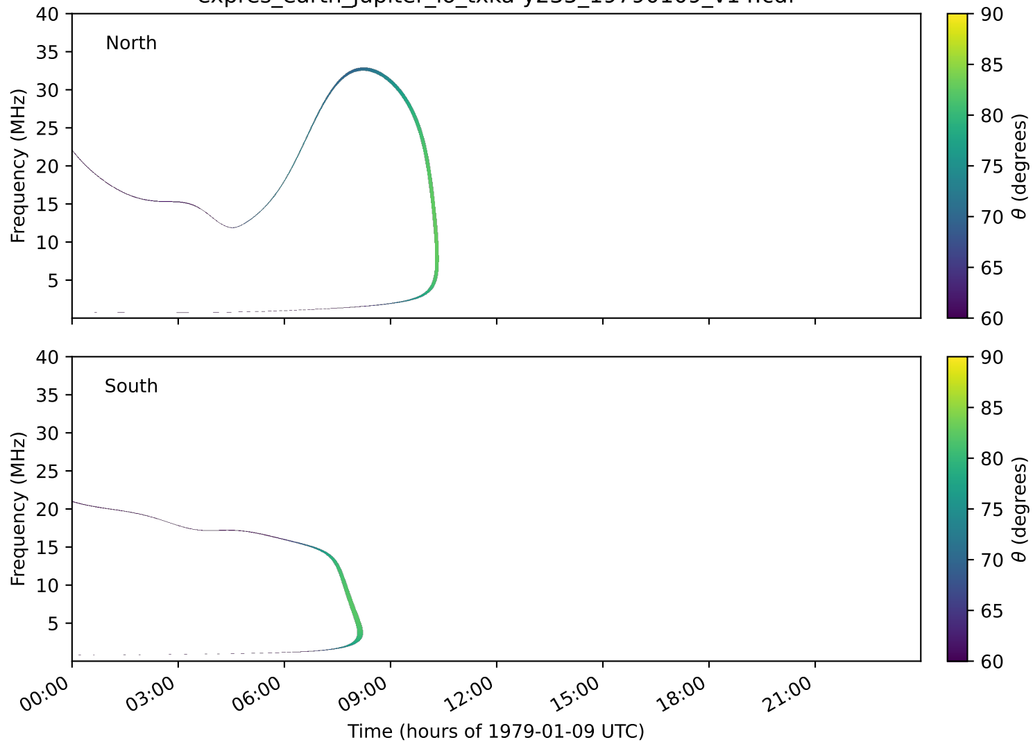
expres_earth_jupiter_io_txka-y235_19790109_v14.cdf
