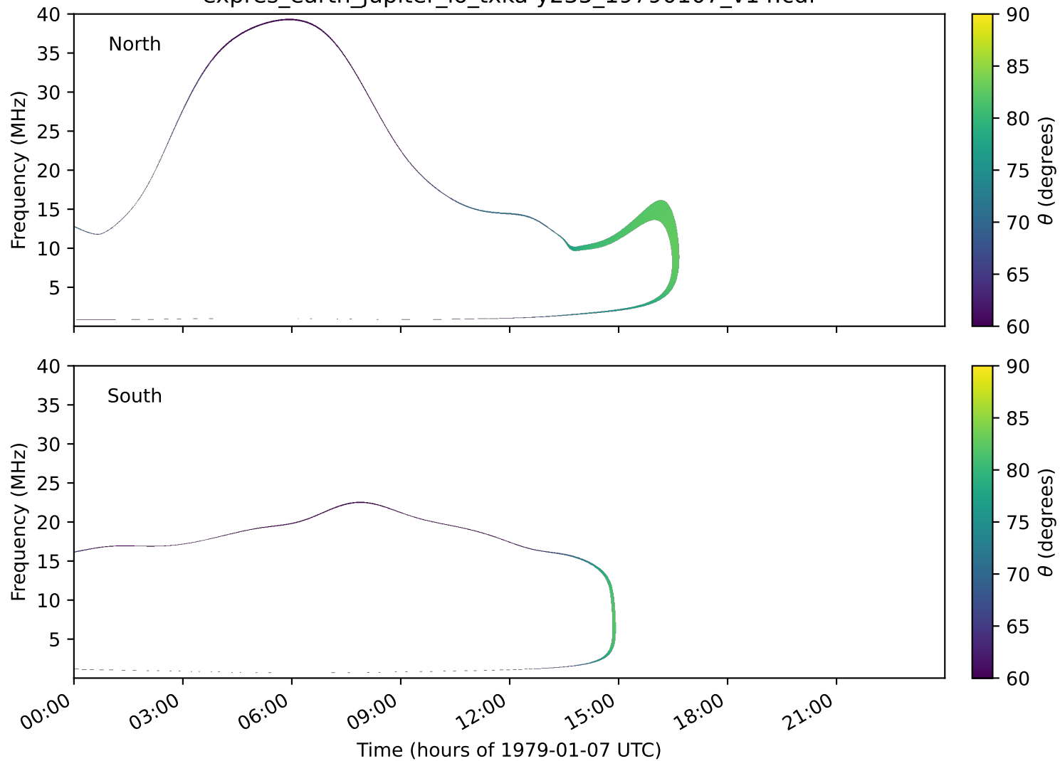
expres_earth_jupiter_io_txka-y235_19790107_v14.cdf
