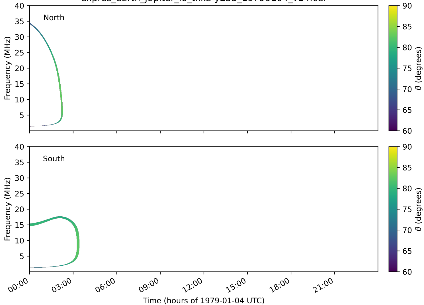
expres_earth_jupiter_io_txka-y235_19790104_v14.cdf
