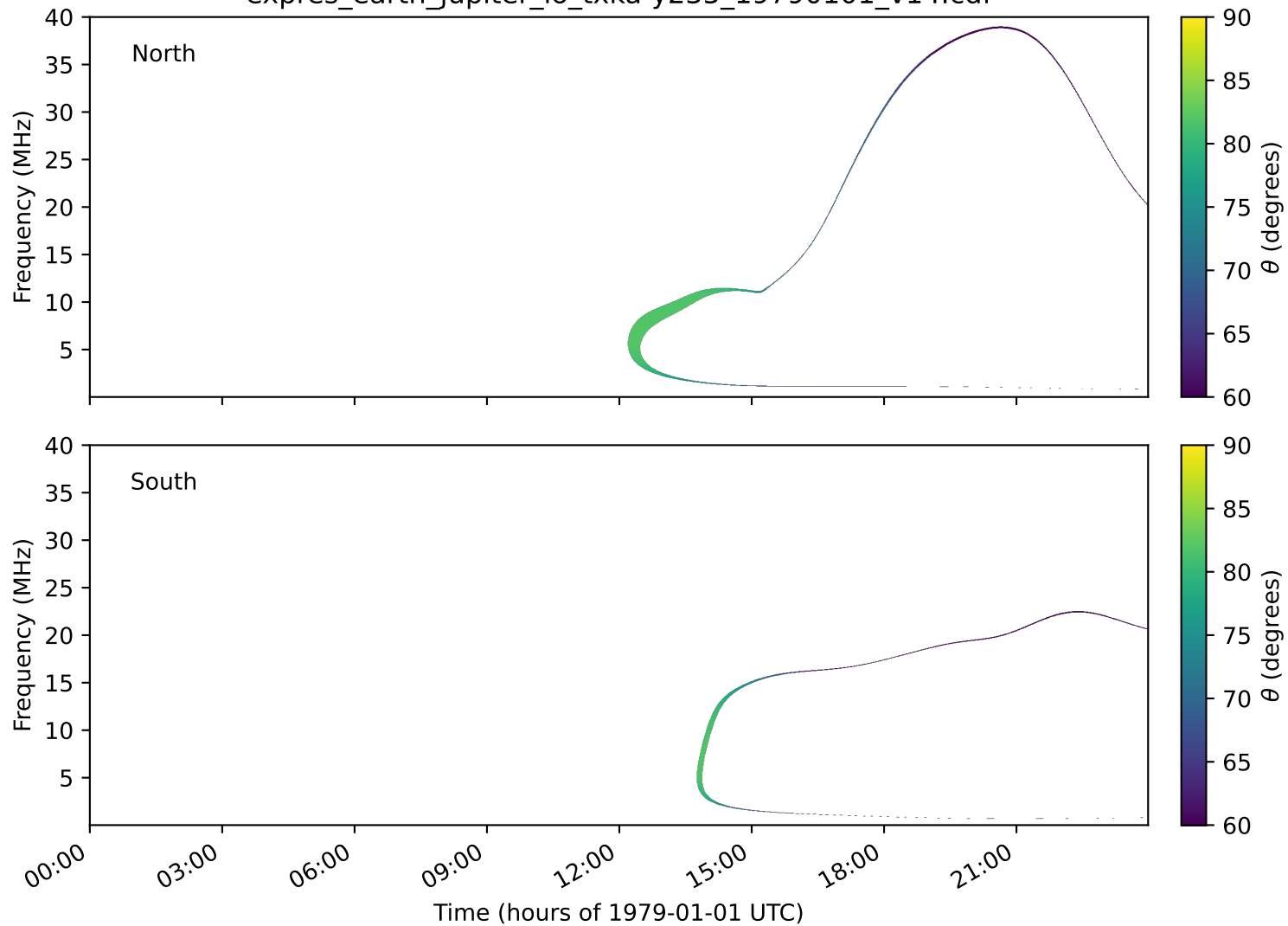
expres_earth_jupiter_io_txka-y235_19790101_v14.cdf
