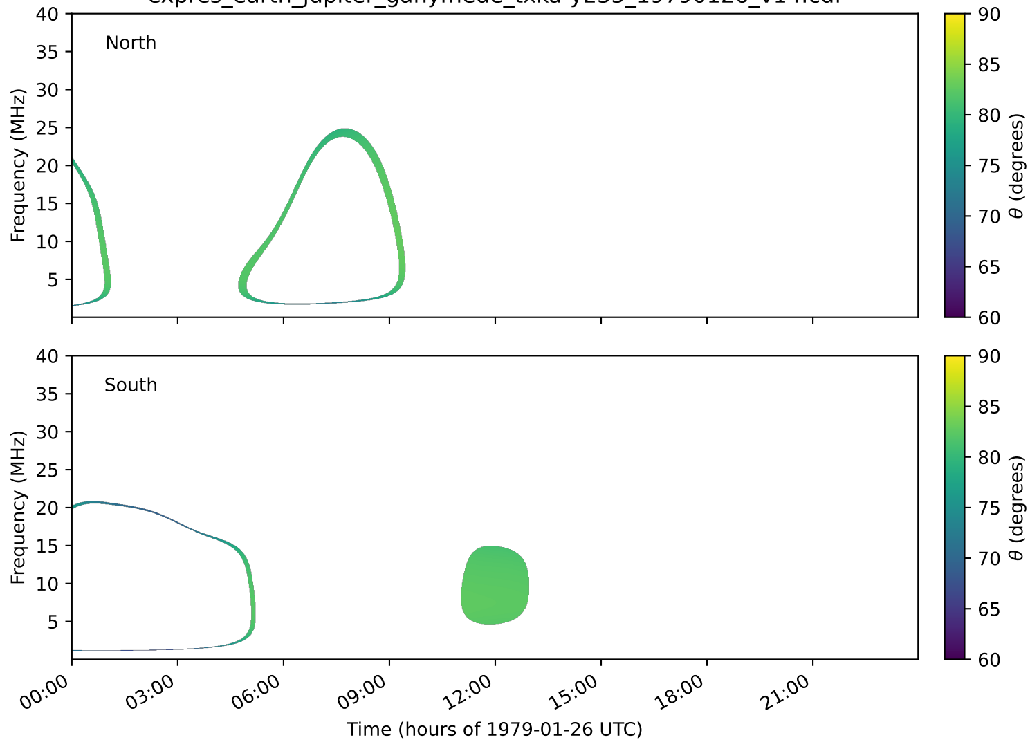
expres_earth_jupiter_ganymede_txka-y235_19790126_v14.cdf
