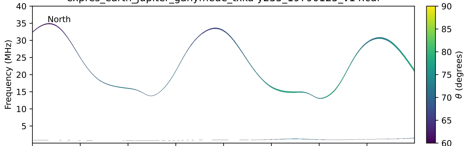
expres_earth_jupiter_ganymede_txka-y235_19790125_v14.cdf
