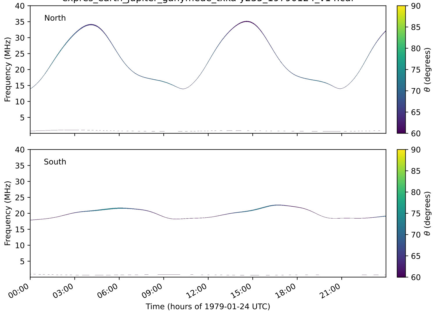
expres_earth_jupiter_ganymede_txka-y235_19790124_v14.cdf
