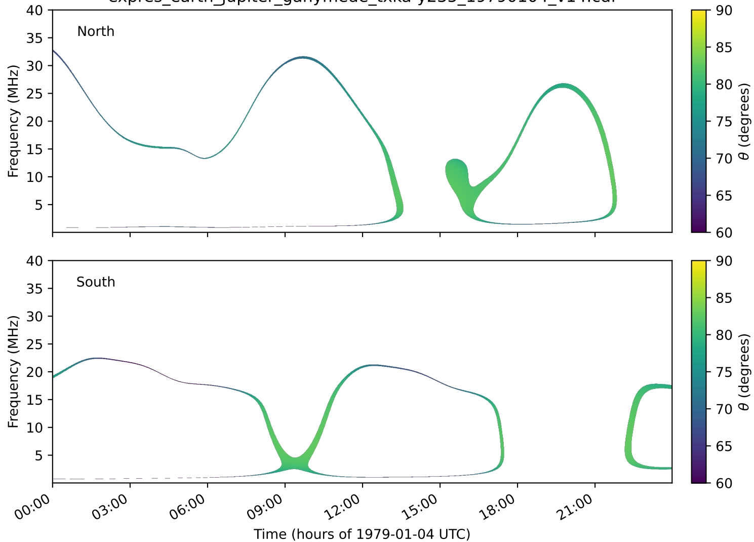
expres_earth_jupiter_ganymede_txka-y235_19790104_v14.cdf
