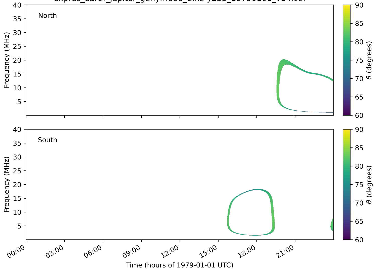
expres_earth_jupiter_ganymede_txka-y235_19790101_v14.cdf
