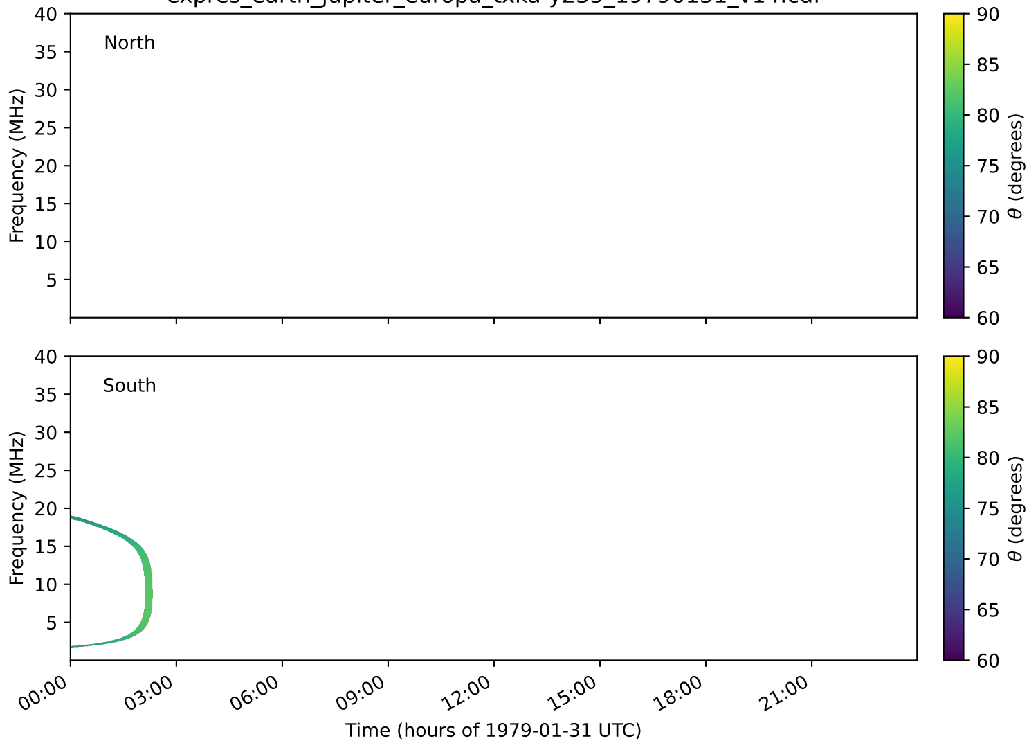
expres_earth_jupiter_europa_txka-y235_19790131_v14.cdf
