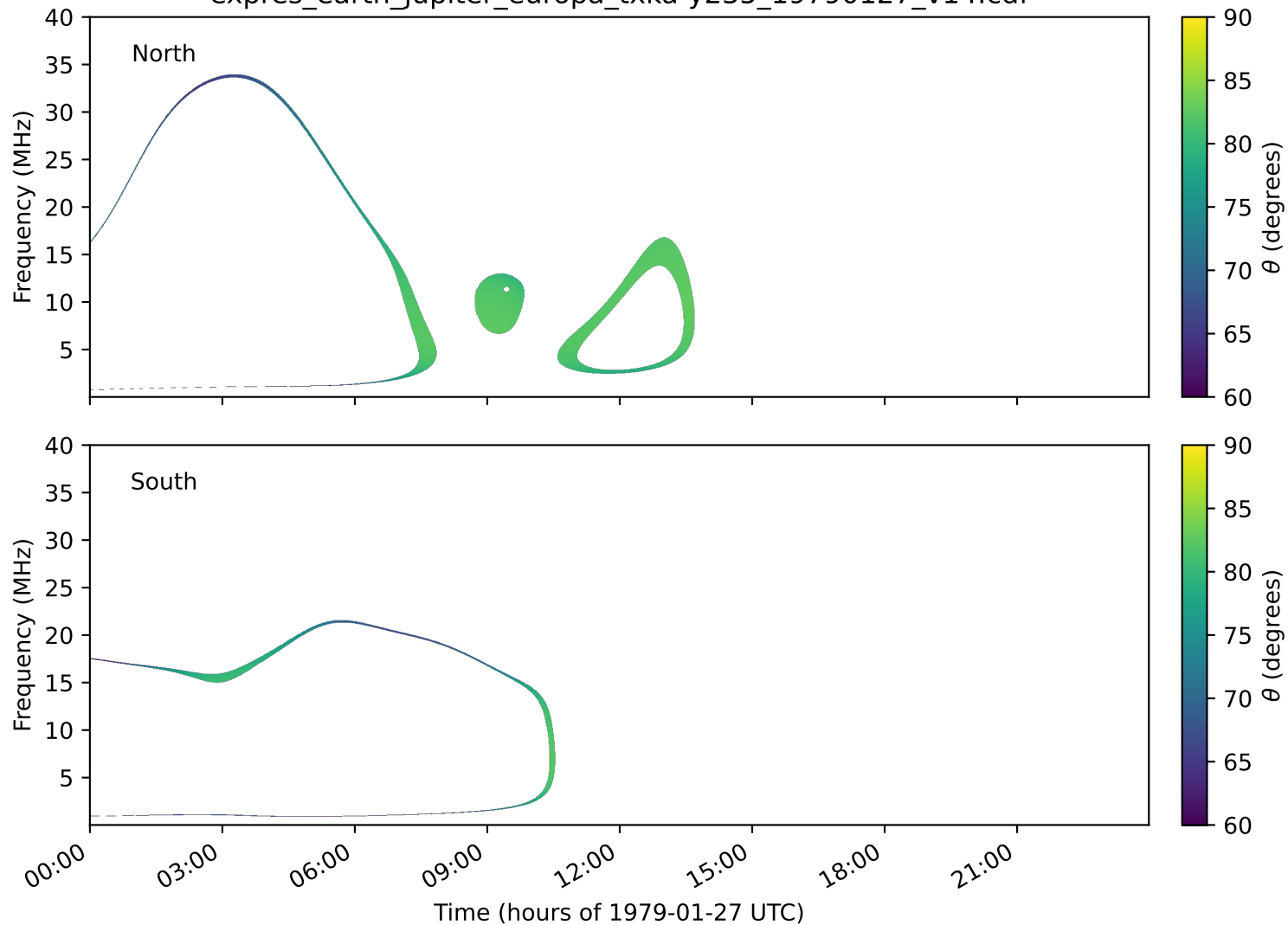
expres_earth_jupiter_europa_txka-y235_19790127_v14.cdf
