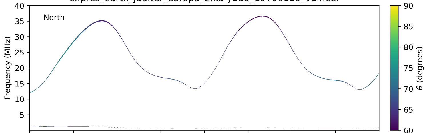
expres_earth_jupiter_europa_txka-y235_19790119_v14.cdf
