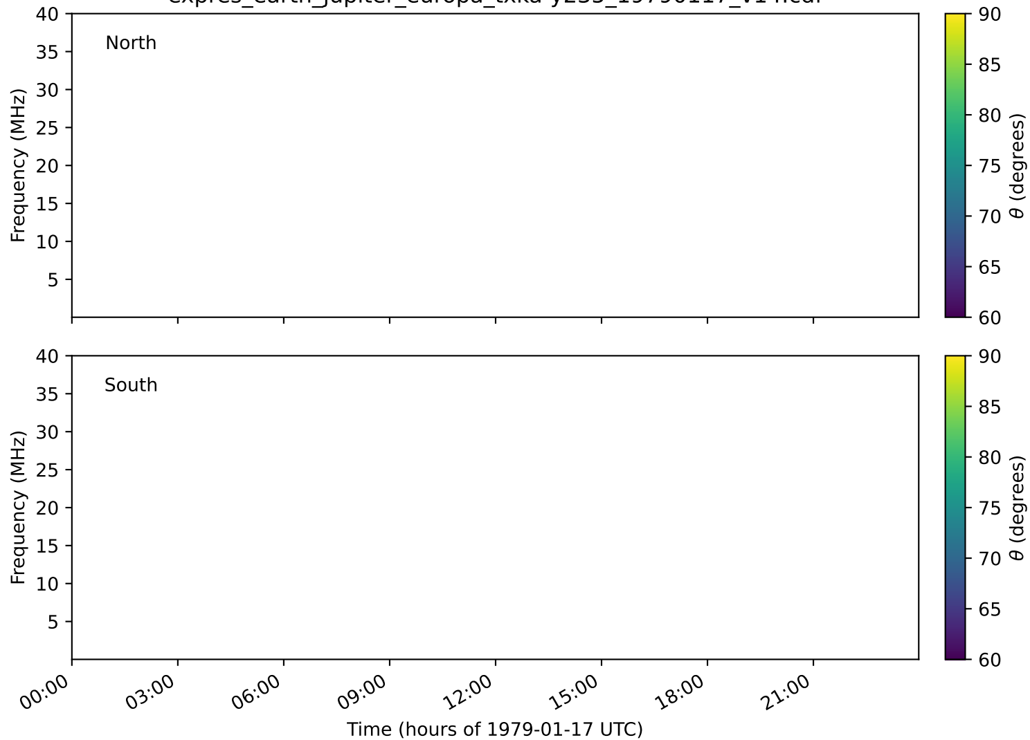
expres_earth_jupiter_europa_txka-y235_19790117_v14.cdf
