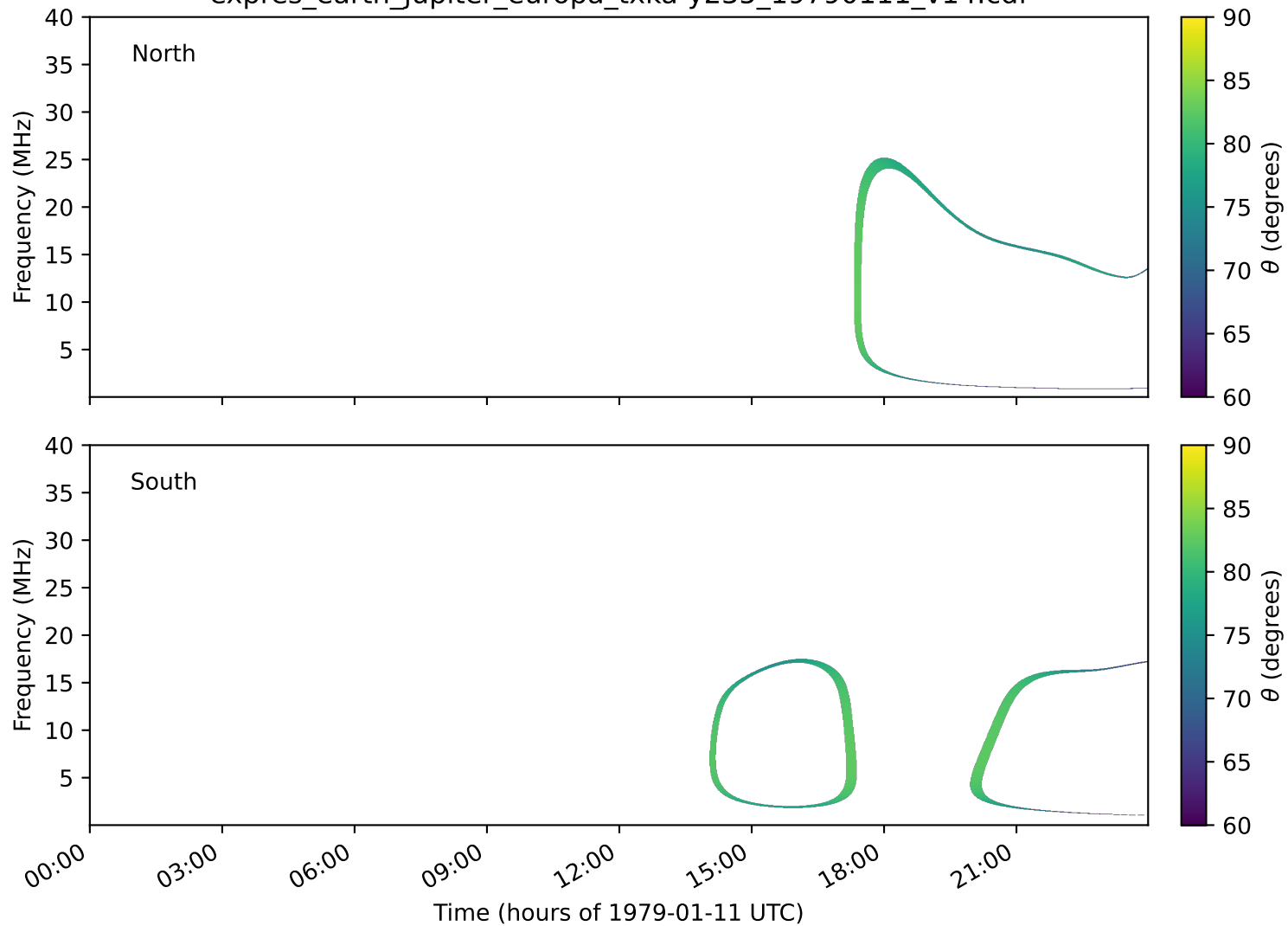
expres_earth_jupiter_europa_txka-y235_19790111_v14.cdf
