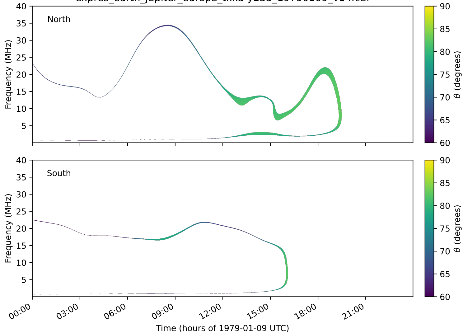
expres_earth_jupiter_europa_txka-y235_19790109_v14.cdf
