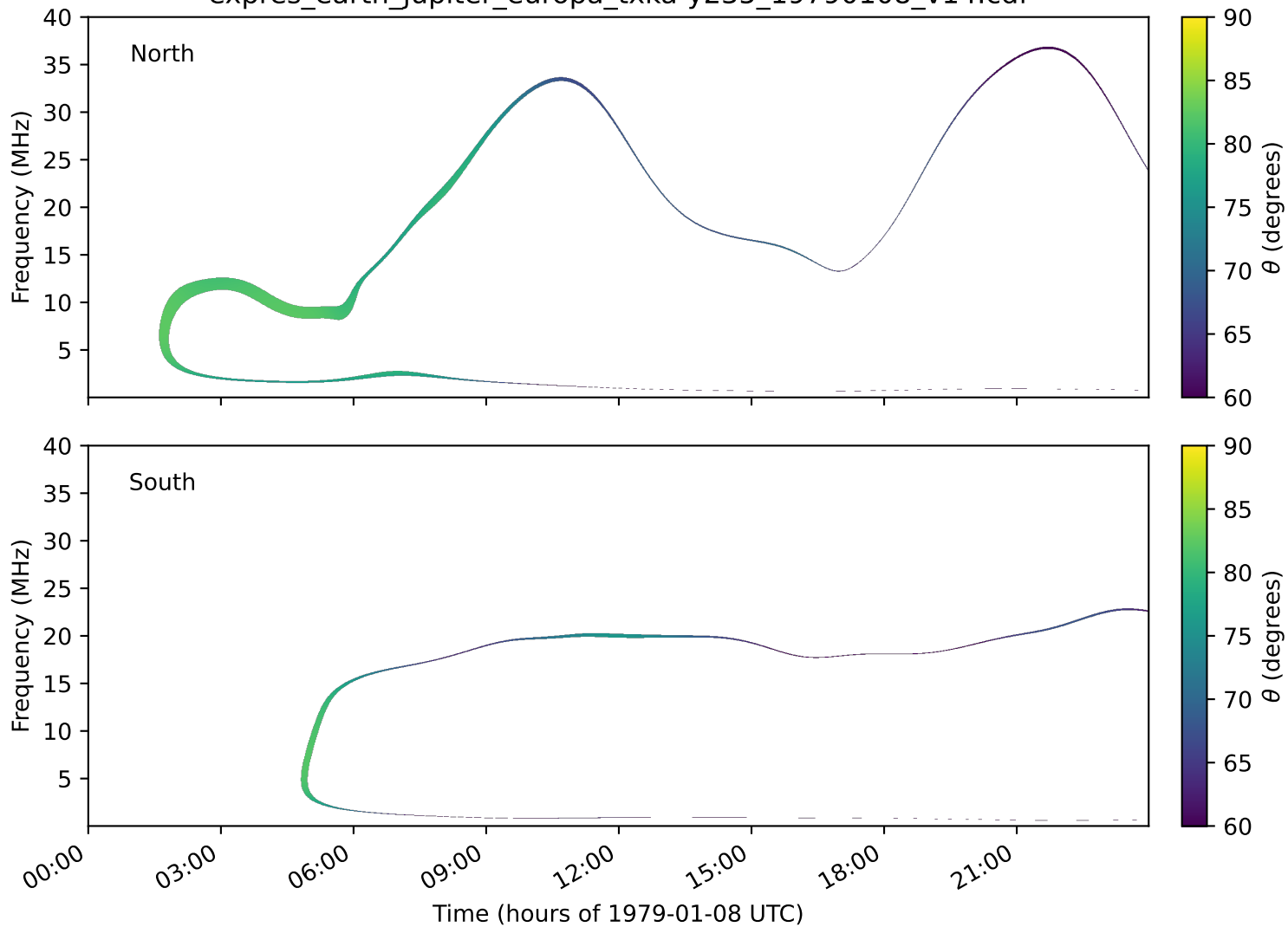
expres_earth_jupiter_europa_txka-y235_19790108_v14.cdf
