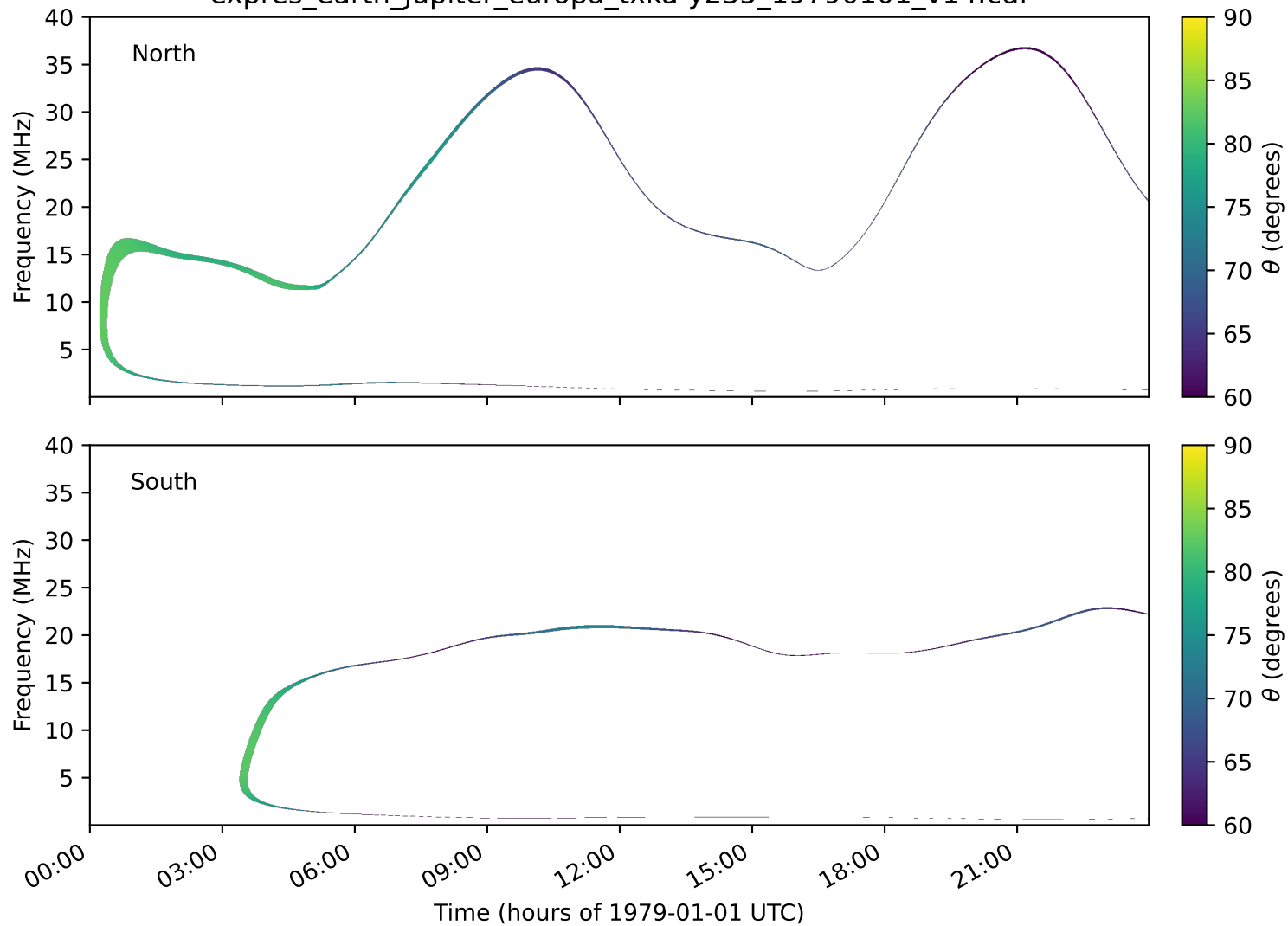
expres_earth_jupiter_europa_txka-y235_19790101_v14.cdf
