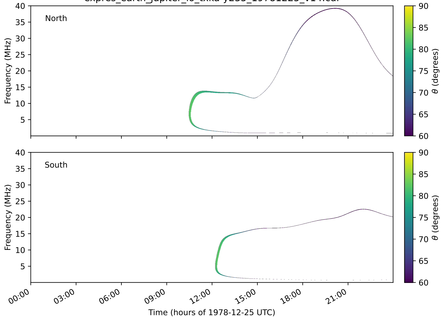
expres_earth_jupiter_io_txka-y235_19781225_v14.cdf
