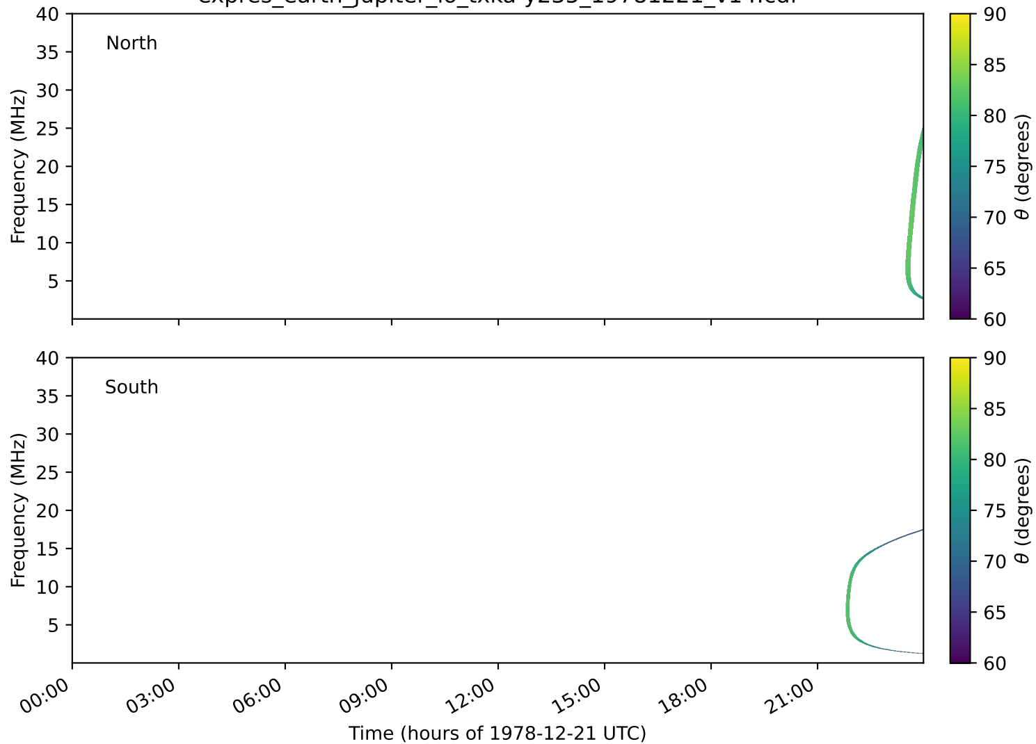
expres_earth_jupiter_io_txka-y235_19781221_v14.cdf
