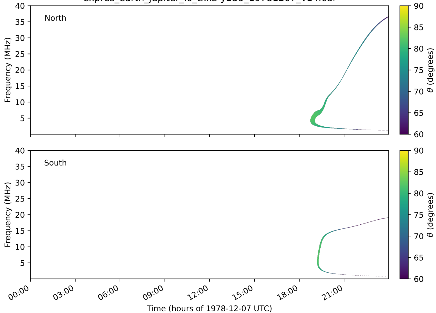
expres_earth_jupiter_io_txka-y235_19781207_v14.cdf
