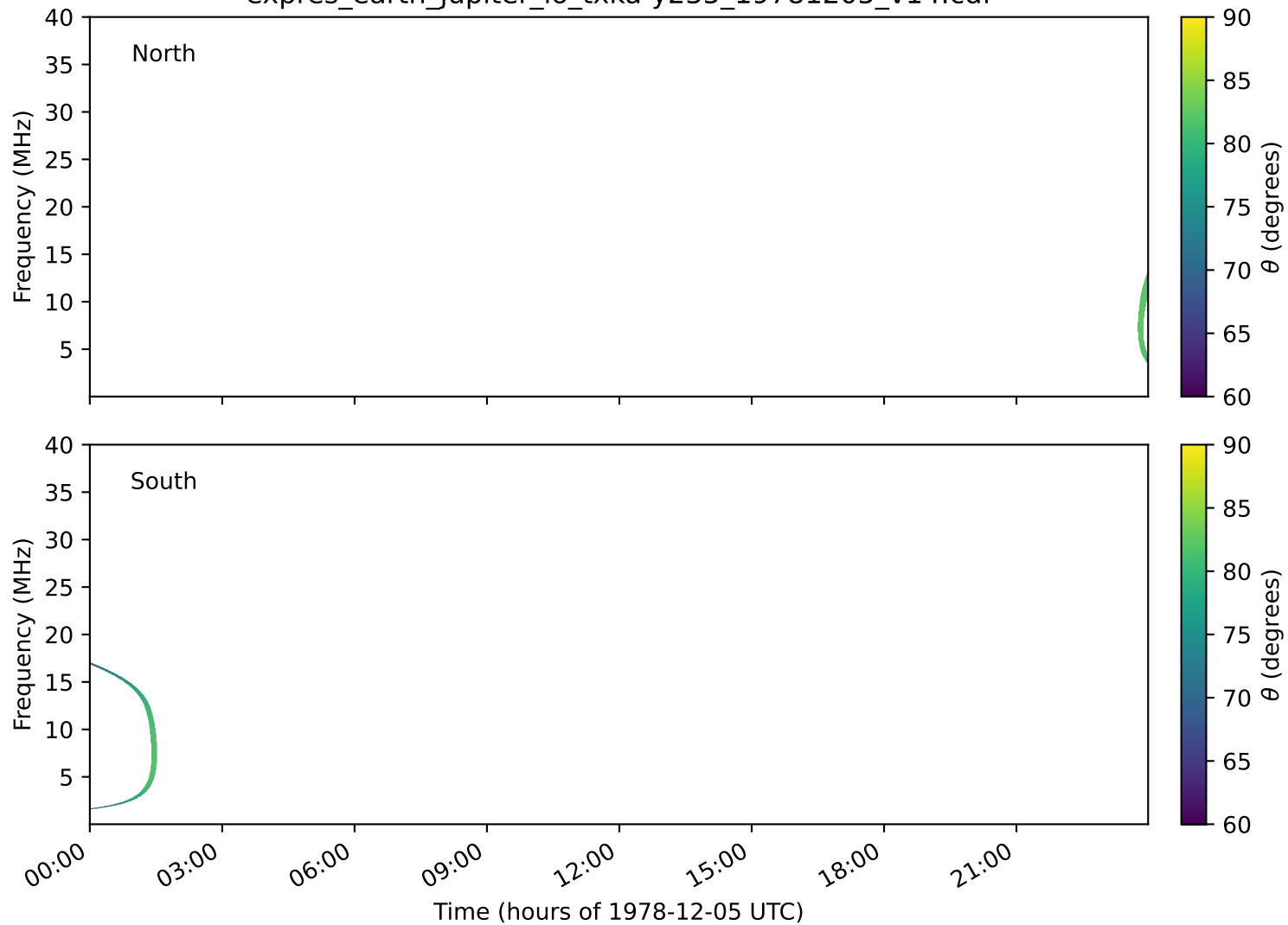
expres_earth_jupiter_io_txka-y235_19781205_v14.cdf
