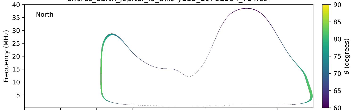
expres_earth_jupiter_io_txka-y235_19781204_v14.cdf
