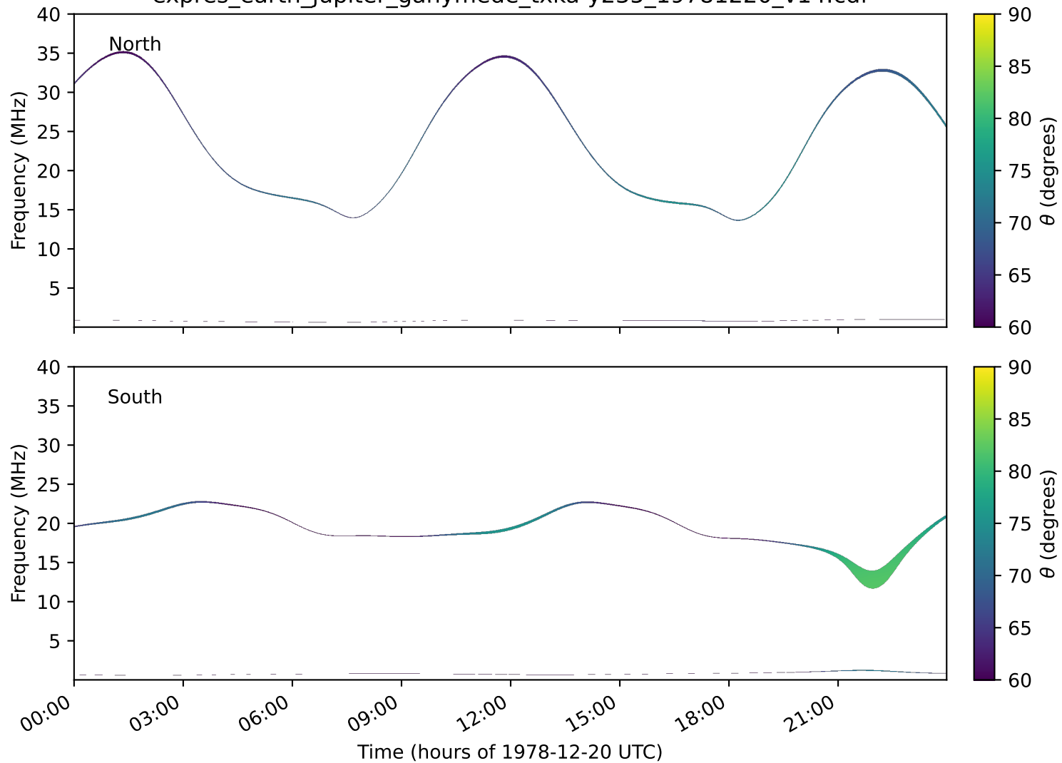
expres_earth_jupiter_ganymede_txka-y235_19781220_v14.cdf
