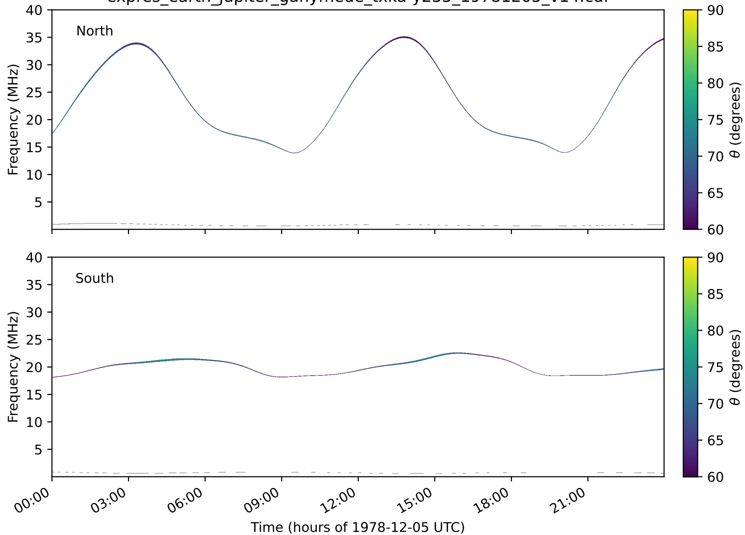
expres_earth_jupiter_ganymede_txka-y235_19781205_v14.cdf
